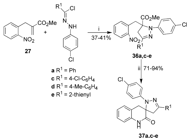
Scheme 5. Reagents and conditions: (a) Et 3 N, C 6 H 6 , reflux, 5 d; (b) Fe/AcOH, reflux, 3 h.
