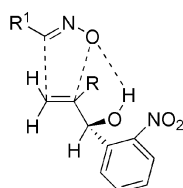
Figure 1. Hydrogen-bonded transition state favoring the formation of the syn isomer.
