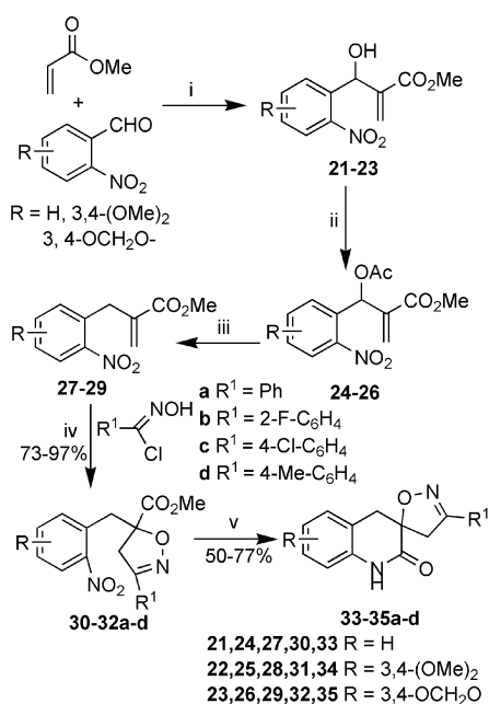
Scheme 4. Reagents and conditions: (i) DABCO, neat, room temp., 10–36 h; (ii) AcCl, pyridine, anhydrous CH 2 Cl 2 , 0 °C to room temp., 2–3 h; (iii) DABCO, THF/H 2 O, room temp., 15 min, then NaBH 4 , room temp., 5 min; (iv) Et 3 N, anhydrous diethyl ether, –78 °C to room temp., 3–4 h; (v) In/HCl, 70 °C, 5–7 min.
