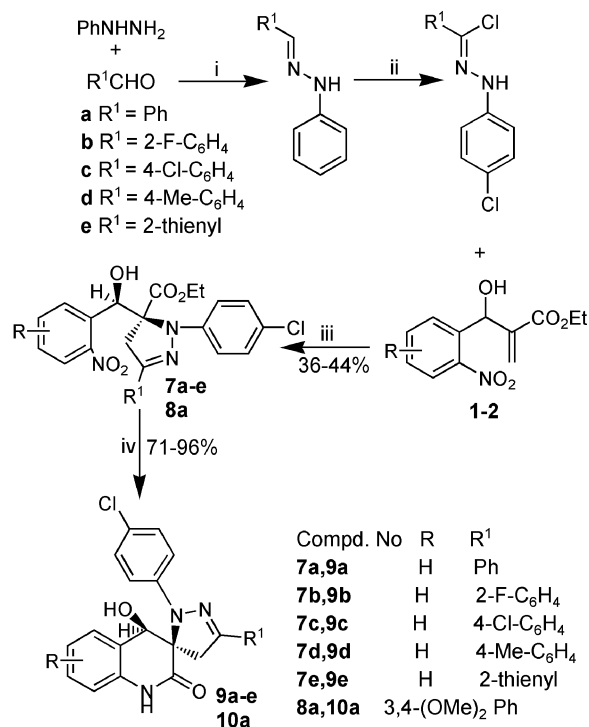
Scheme 2. Reagents and conditions: (i) \text{C}_6\text{H}_6 , room temp. to reflux, 2–15 min; (ii) NCS, DMF, room temp., 30 min to 1 h; (iii) \text{Et}_3\text{N} , anhydrous \text{C}_6\text{H}_6 , reflux, 5 d; (iv) Fe/AcOH, reflux, 3 h.
