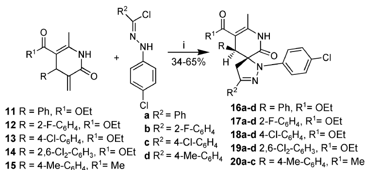
Scheme 3. Reagents and conditions: (i) Anhydrous C 6 H 6 , reflux, 5 d.
