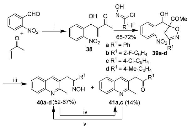
Scheme 6. Reagents and conditions: (i) DABCO, neat, 0 °C, 10 min; (ii) \text{Et}_3\text{N} , anhydrous diethyl ether, –78 °C to room temp., 3 h; (iii) \text{In}/\text{HCl} , 70 °C, 5–7 min; (iv) 35% aqueous \text{HCl} , \text{THF}/\text{H}_2\text{O} , reflux, 1 h; (v) \text{NH}_2\text{OH}\cdot\text{HCl} , \text{NaOAc} , \text{MeOH} , reflux, 1 h.
