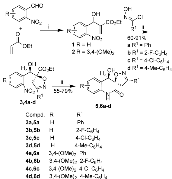
Scheme 1. Reagents and conditions: (i) DABCO, neat, room temp., 10–24 h; (ii) Et 3 N, anhydrous diethyl ether, –78 °C to room temp., 3 h; (iii) In/HCl, 70 °C, THF/H 2 O (3:2), 5–7 min.
