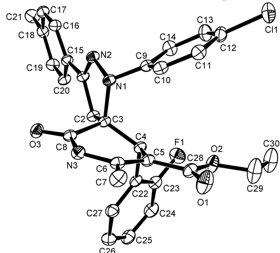
Figure 2. ORTEP structure of 17d . The ellipsoids are drawn at a probability level of 20%.
