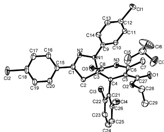
Figure 3. ORTEP structure of 19c with a molecule of chloroform. The ellipsoids are drawn at a probability level of 20%.
